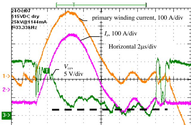
Fig. 10. Differential measurement of V_{sar} (trace 3 V_{ce} ) of CM300DC-24NFM Powerex IGBT using circuit Fig. 4. Trace 3 may have some offset, likely zero is shown by dashed line.
