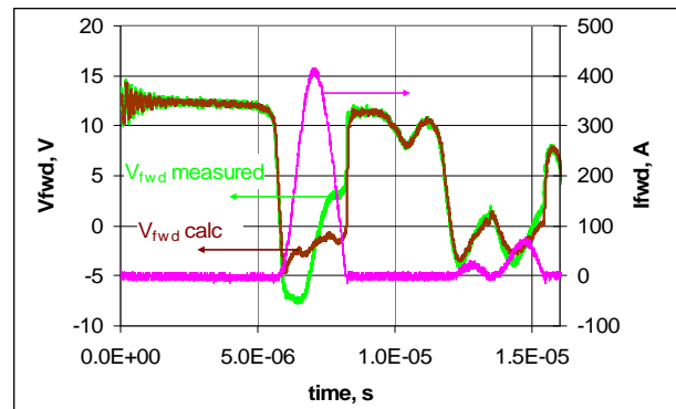
Fig. 8. Trace 2 - Forward drop of FWD IXYS DSEI 2x 61 (negative part). Clamped positive voltage (diode non-conducting) is off-scale. Zener diode capacitance (divider Fig. 4) affects the voltage fall time.
