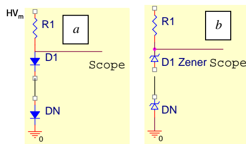
Fig. 1. Schematics of basic nonlinear voltage dividers.
