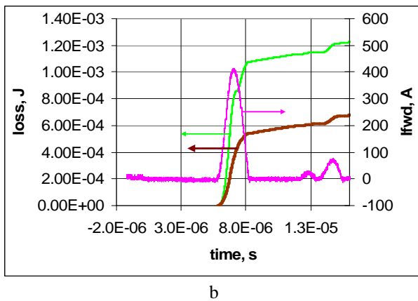
Fig. 9. FWD IXYS DSEI 2x61 losses. Plot a – green trace is measured signal; brown trace is V_{fwd} adjusted for inductive drop LdI_{fwd}/dt (diode assembly inductance assessed at 5 nH). Green and brown curves plot b match their counterparts in plot a. Divider Fig. 7, Floating scope.
